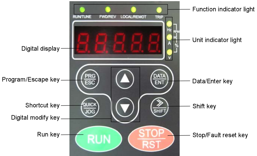
Figure 5.1 Keypad schematic diagrams.
