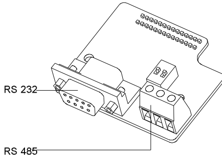
Figure 7.12 Modbus communication card
